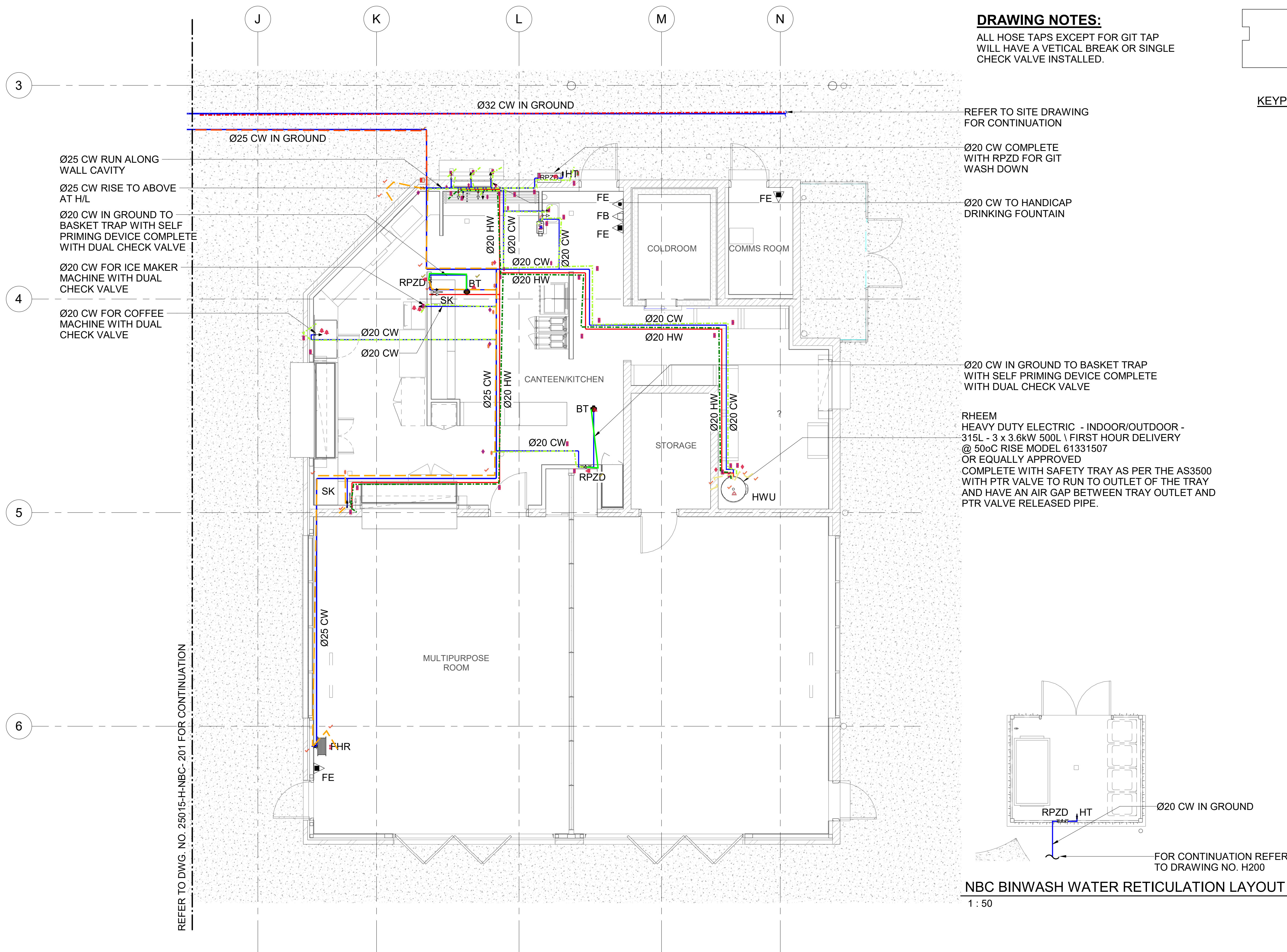
GROUND FLOOR WATER RETICULATION LAYOUT - PART PLAN 3
